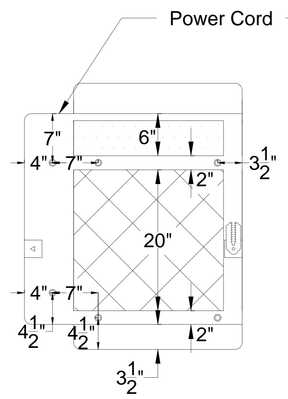
Single Arm
